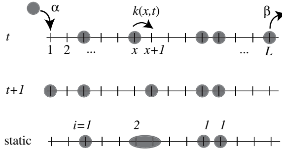
Figure 1. Illustration of the relationship between the TASEP and the hard core lattice gas. In the TASEP particles (grey dots) occupy a one-dimensional lattice, labelled by x = 1, \dots, L . A particle can hop from site x to site x + 1 at rate k(x, t) . The system is coupled to an input and an output reservoir with rates \alpha and \beta , respectively. In the equilibrium binary mixture particles on a lattice occupy one (species i = 1 ) or two (species i = 2 ) lattice sites. The position coordinate of the two particles is taken as the left excluded site.
