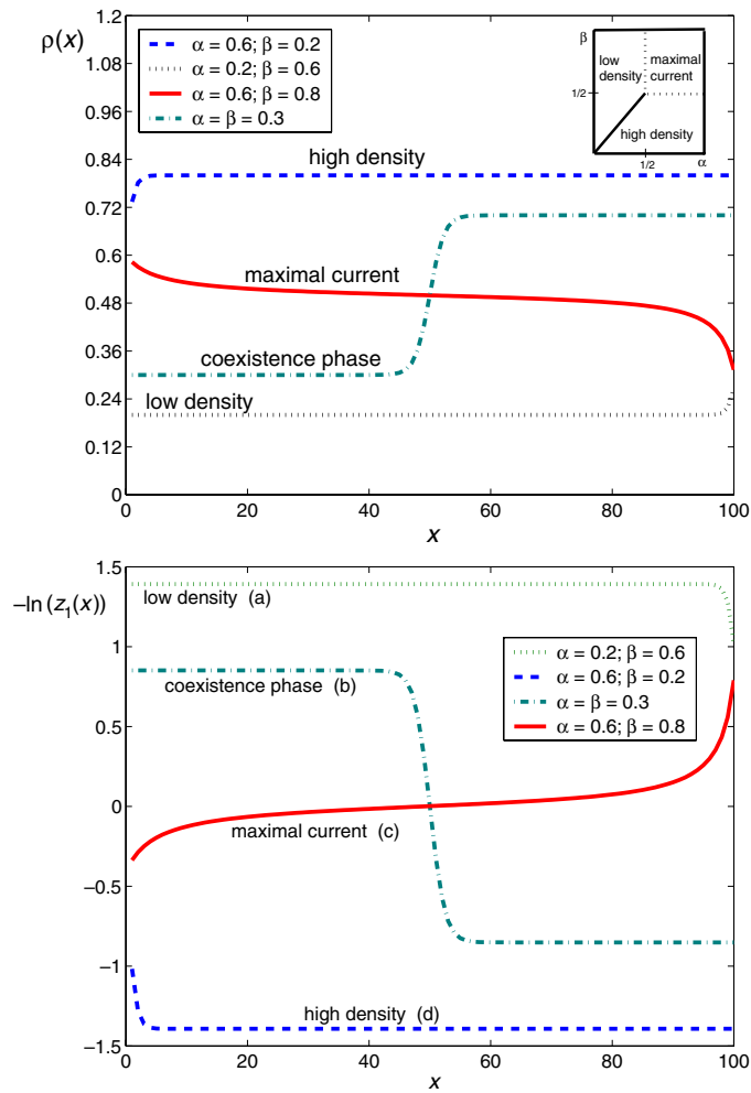
Figure 2. Upper panel. Representative density profiles \rho(x) as a function of position x for the TASEP with open boundaries. Results are obtained from mean-field theory for a system of size L = 100 in the high density phase ( \alpha = 0.6, \beta = 0.2 , dashed line), low density phase ( \alpha = 0.2, \beta = 0.6 , dotted line), maximal current phase ( \alpha = 0.6, \beta = 0.8 , solid line) and coexistence between high and low density phases ( \alpha = \beta = 0.3 , dash-dotted line). The inset shows the out-of-equilibrium phase diagram of the TASEP as a function of \alpha and \beta including high density, low density, maximal current and coexistence (thick line) phases. Lower panel. Local fugacities z_1(x) of small particles that generate the same density profiles for species 1, \rho_1(x) , as shown in the upper panel.
